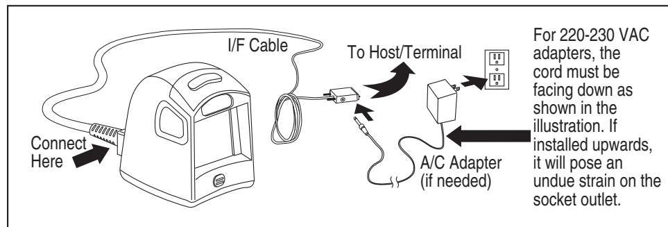
Figure 1. RS-232 Serial or USB Connection using A/C Adapter
